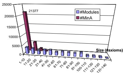
Figure 2: Module and MinA size distribution.
