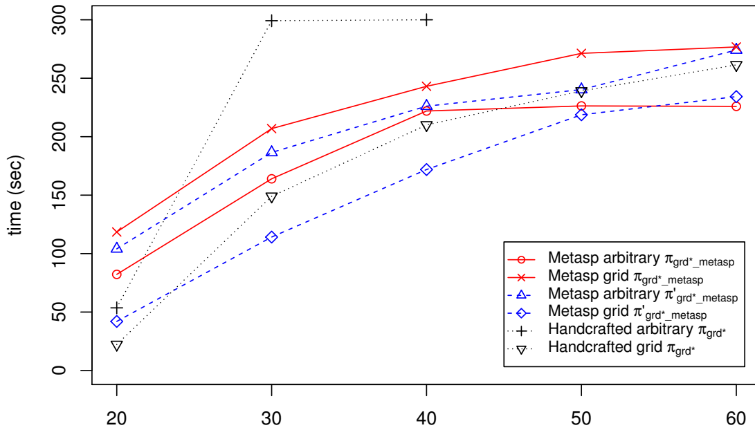
Fig. 4. Average computation time for resolution-based grounded semantics
