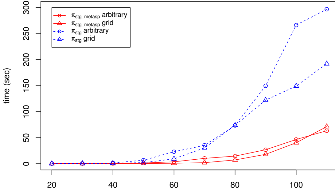
Fig. 3. Average computation time for stage semantics.
